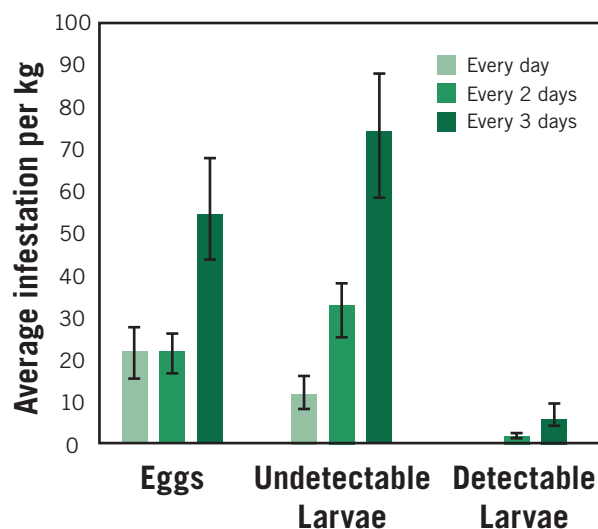
Figure 7. The number of SWD eggs, undetectable larvae (1 st and 2 nd instars) and detectable larvae (3 rd instar) per kilogram of raspberries when harvested daily, every 2 days, and every 3 days.
