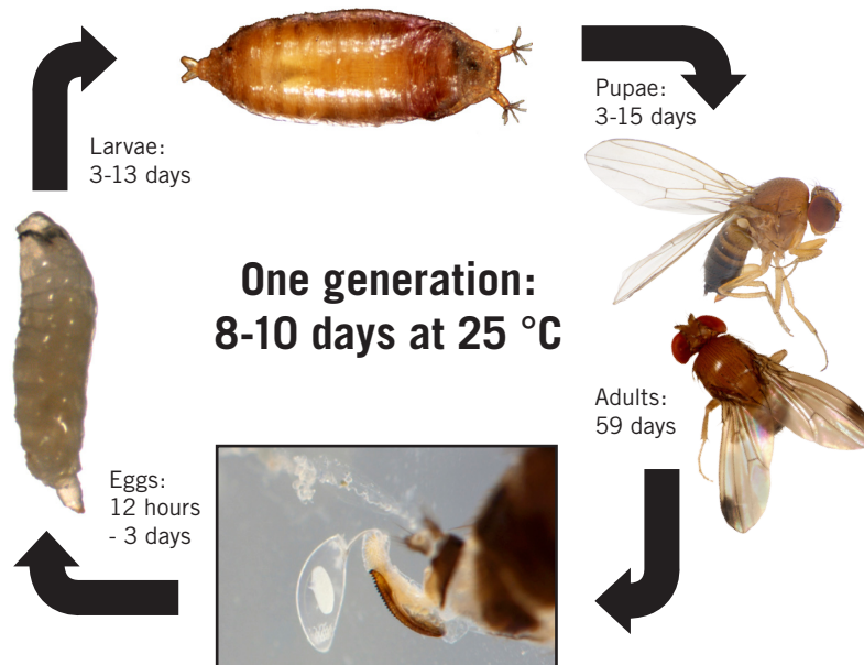
Figure 3. The lifecycle of SWD.
